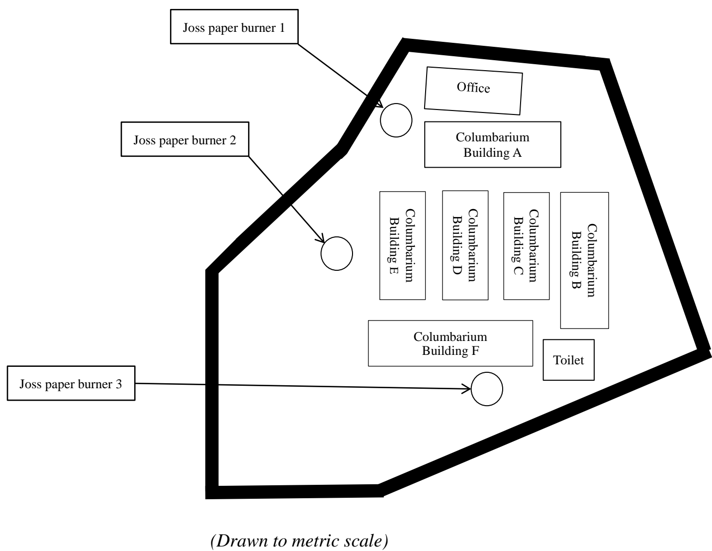
Proposed Layout Plan (Plan No. 002)
