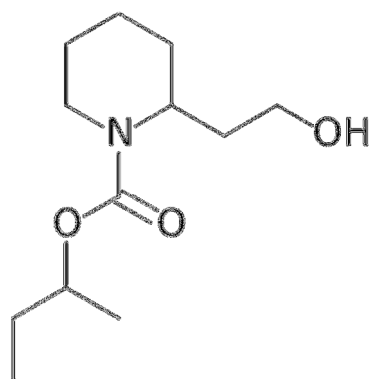
Fig. 1 Chemical structure of Icaridin
