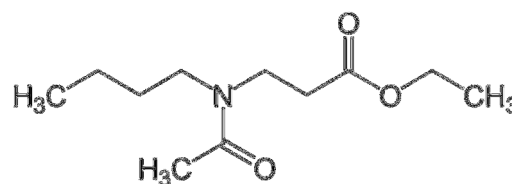
Fig. 2 Chemical structure of IR3535
