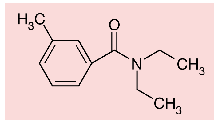
Figure 1. Chemical structure of N,N-Diethyl-3-methylbenzamide, DEET.
