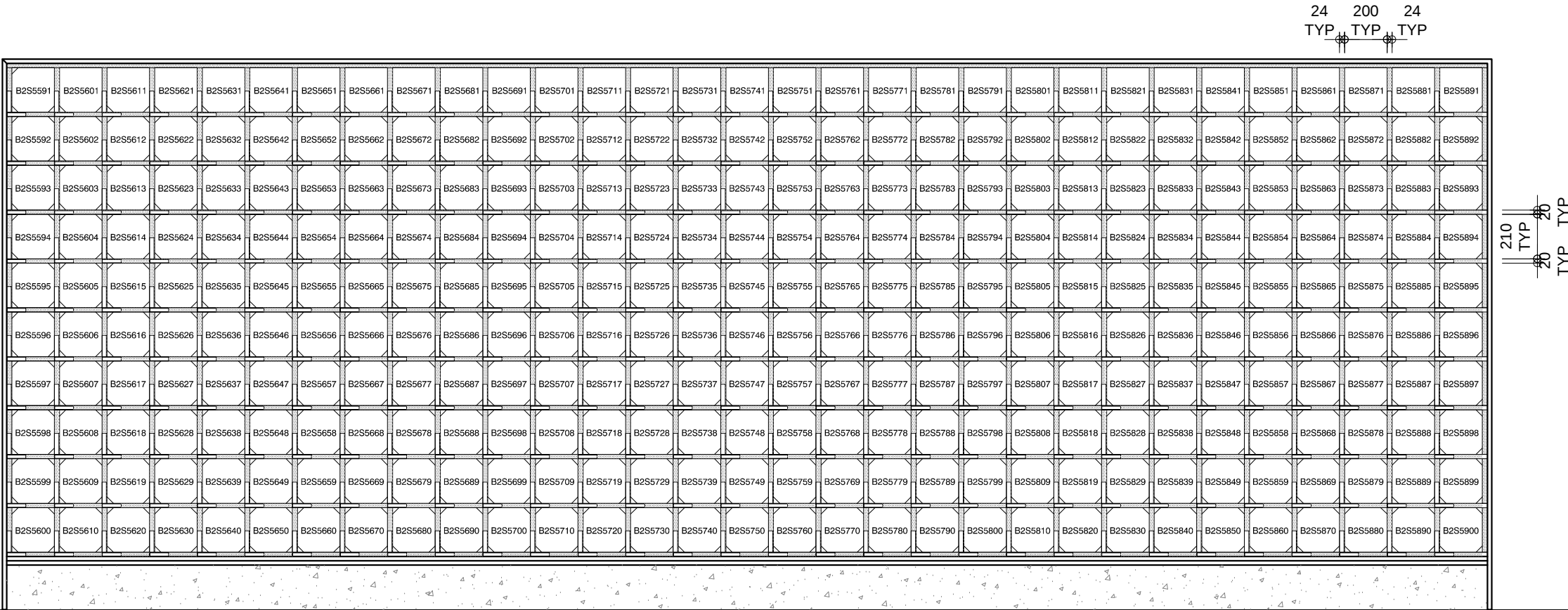
B2S5591 ~ B2S5900 二樓立面圖18 Second Floor Elevation Map 18
