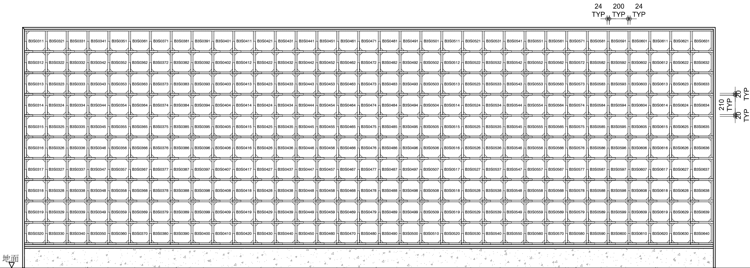
B3S0311 ~ B3S0640 三樓立面圖20 Third Floor Elevation Map 20
