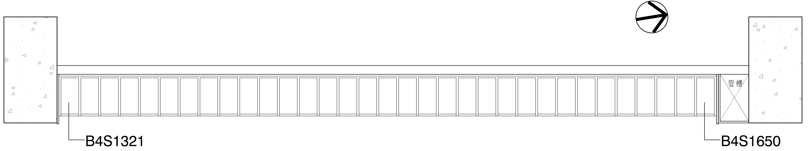
四樓平面圖41 Fourth Floor Plan Map 41
