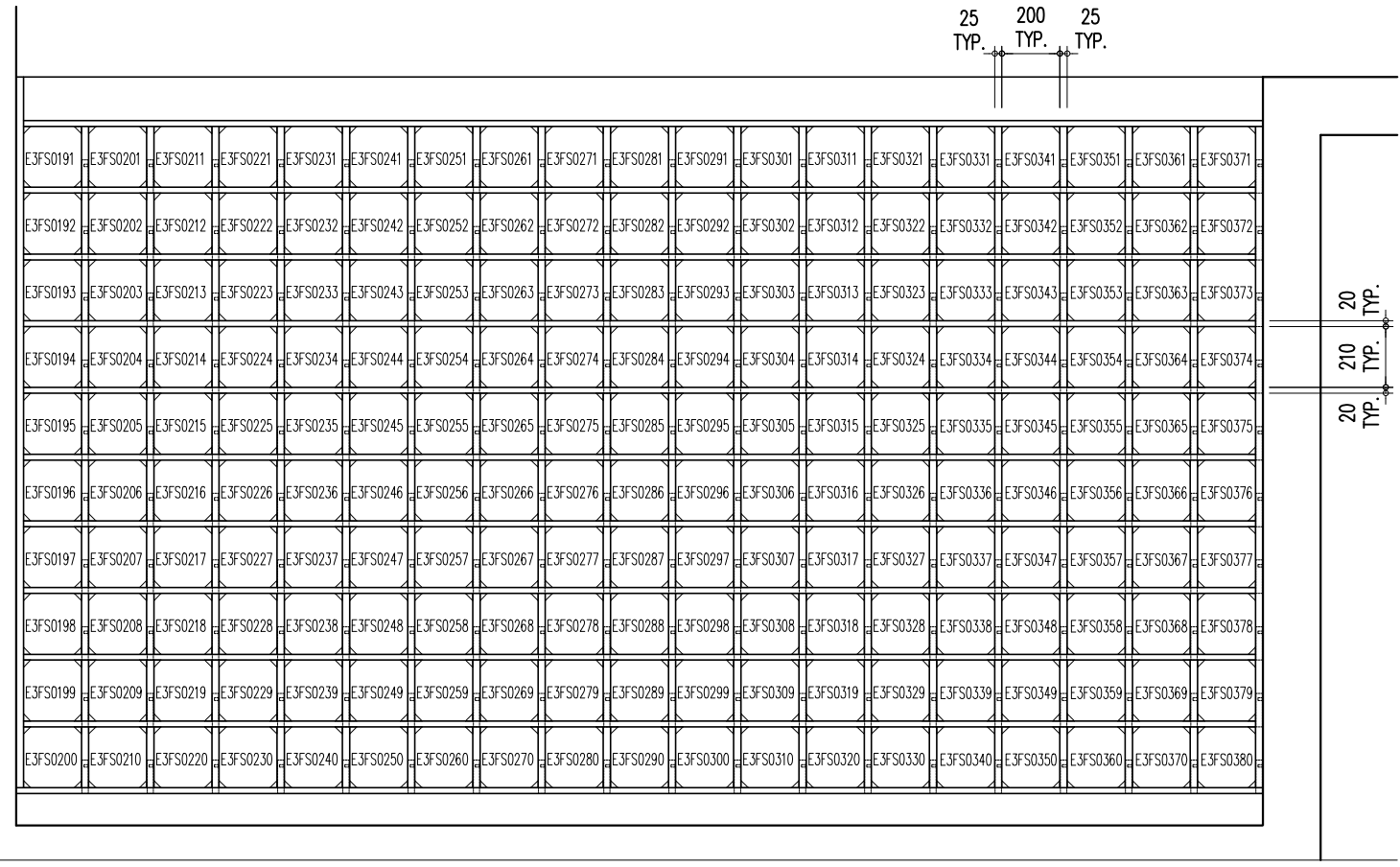
E.3FS0191 ~ E.3FS0380 3/F ELEVATION A
