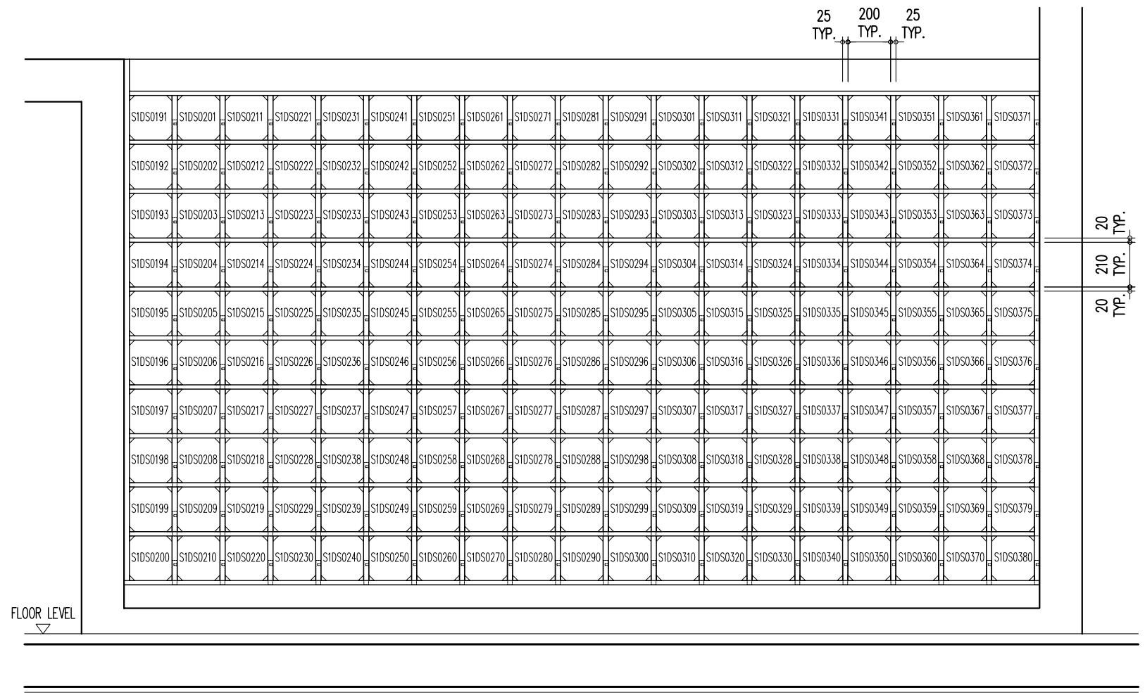
S1DS0191 ~ S1DS0380 1/F ELEVATION A
