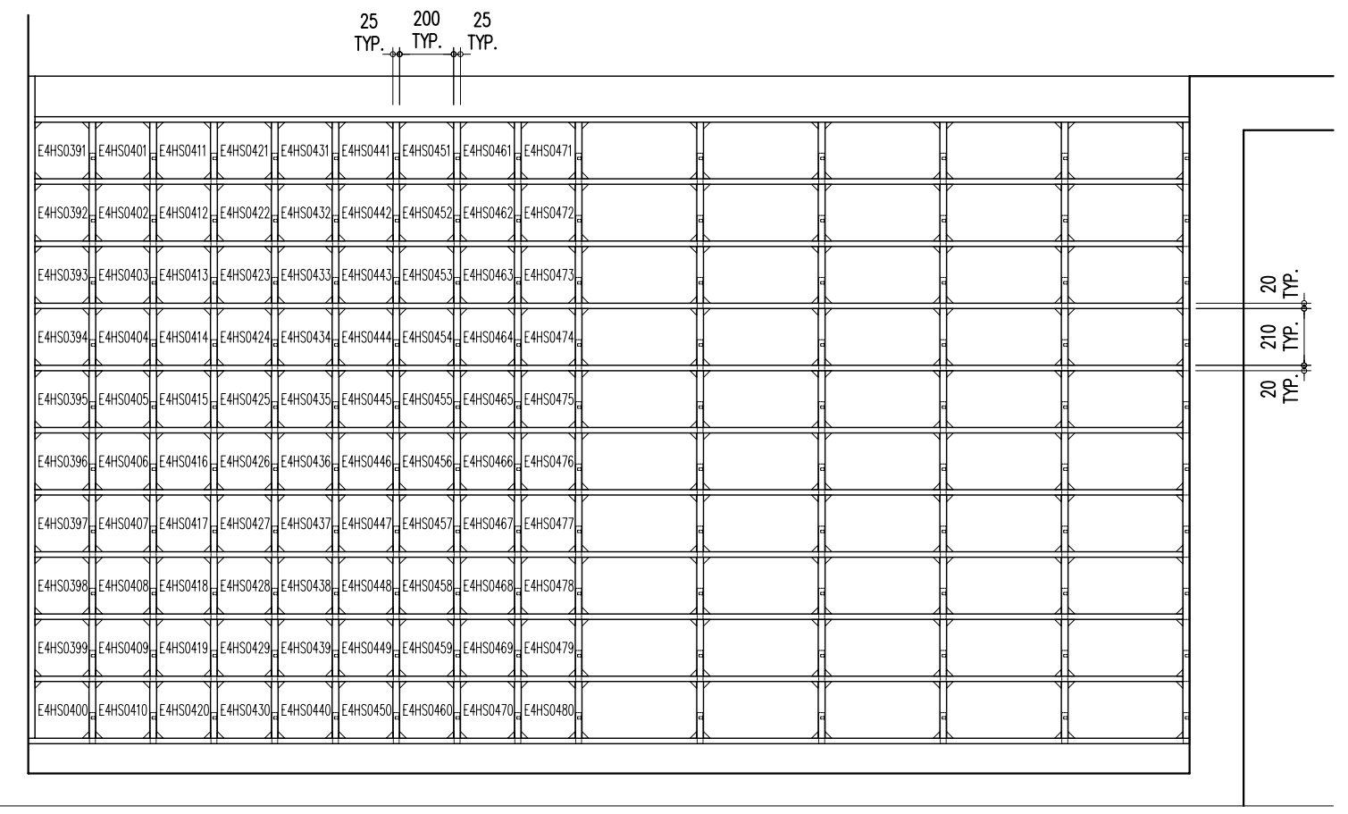
E4HS0391 ~ E4HS0480 4/F ELEVATION A
