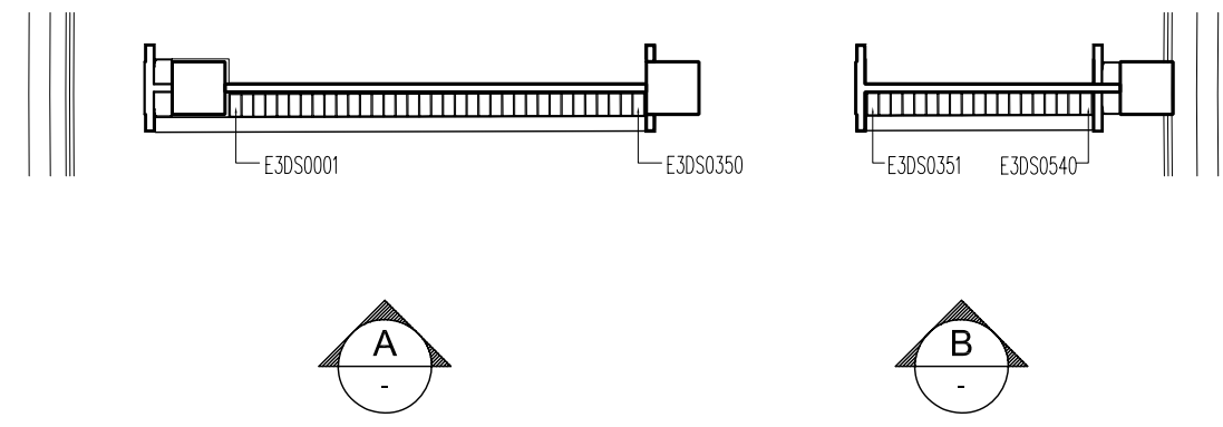
3/F FLOOR PLAN
